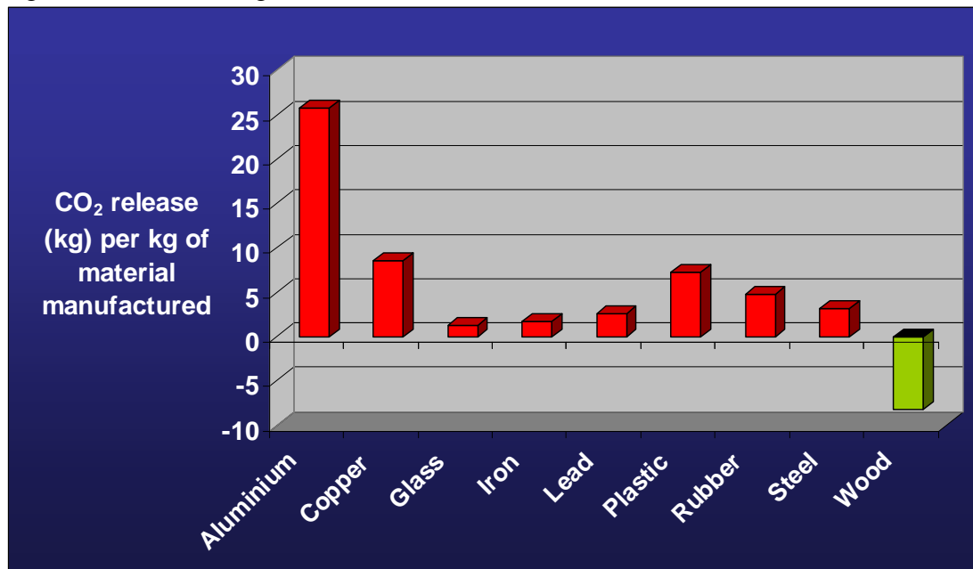
Figure 3. Greenhouse gas release in manufacture of construction materials
